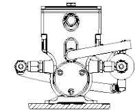
MONTAGE NON CONFORME WRONG MOUNTING
