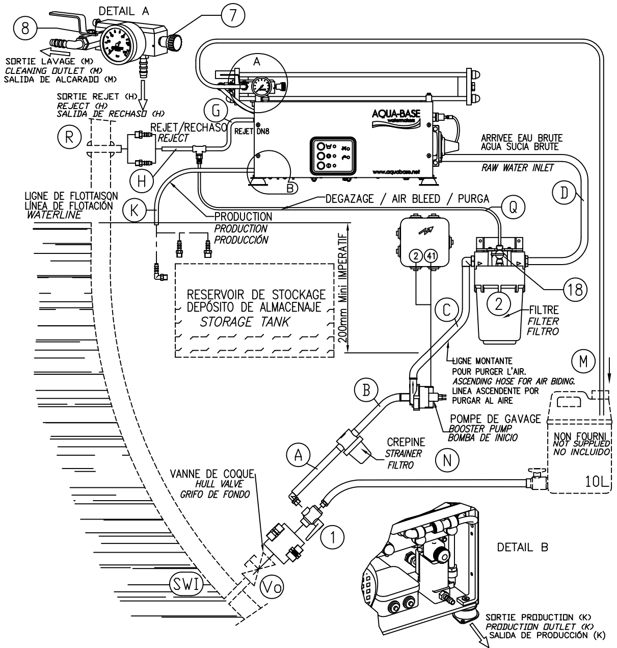
Fig15. INSTALLATION A BORD / ON BOARD INSTALLATION LAYOUT / INSTALACION
